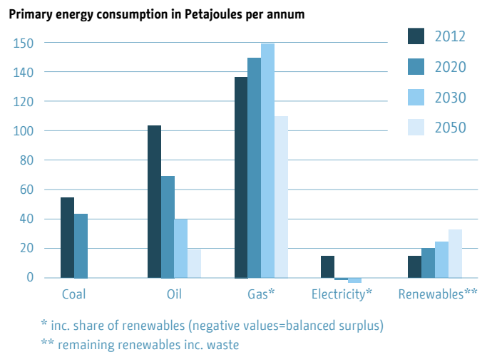
Figure 13: Target values for absolute primary and final energy consumption by energy source 2012–2050
