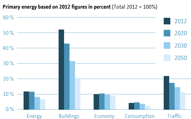
Figure 12: Fields of action as a percentage of primary energy consumption and CO 2 polluter balance 2012–2050
